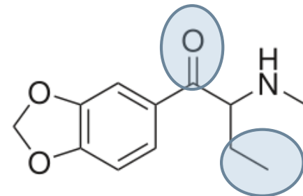
Mephedrone
