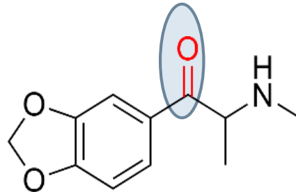
Methylone
