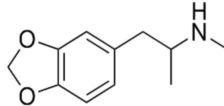
ECSTASY
